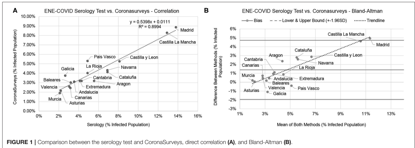
FIGURE 1 | Comparison between the serology test and CoronaSurveys, direct correlation (A), and Bland-Altman (B). TABLE 1 | Percentage (and 95% confidence interval) of infected population per region according to the ENE-COVID serology study (14), CoronaSurveys, and Covid19Impact (11) (symptom-only model).
