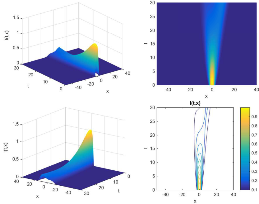
Figure 3: Numerical simulations of the solution I(t, x) . Parameters are d_S = 0.3 , d_I = 0.2 , h = 0.2 , \tau = 1 , \alpha = 0.1 , \mu = 0.1 and \beta = 0.5 .
