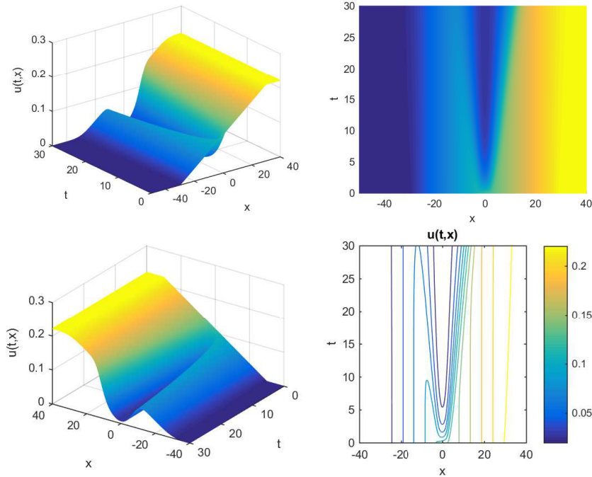
Figure 4: Numerical simulations of the solution u(t, x) . Parameters are d_S = 0.3 , d_I = 0.2 , h = 0.2 , \tau = 1 , \alpha = 0.1 , \mu = 0.1 and \beta = 0.5 .
