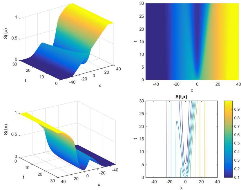
Figure 2: Numerical simulations of the solution S(t, x) . Parameters are d_S = 0.3 , d_I = 0.2 , h = 0.2 , \tau = 1 , \alpha = 0.1 , \mu = 0.1 and \beta = 0.5 . As we can see in the figure, the wave is not monotone.
