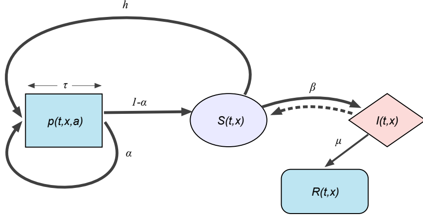
Figure 1: Schematic representation of the interactions between the compartments of the epidemiological model.
