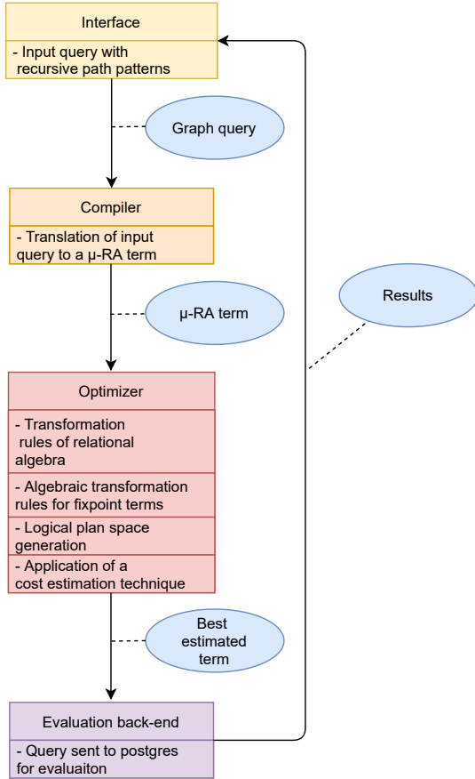
Fig. 1: Architecture of the system.
