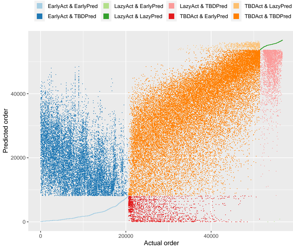
Figure 3: Comparison of the actual and predicted orders of blocks, under Algorithm 1.
