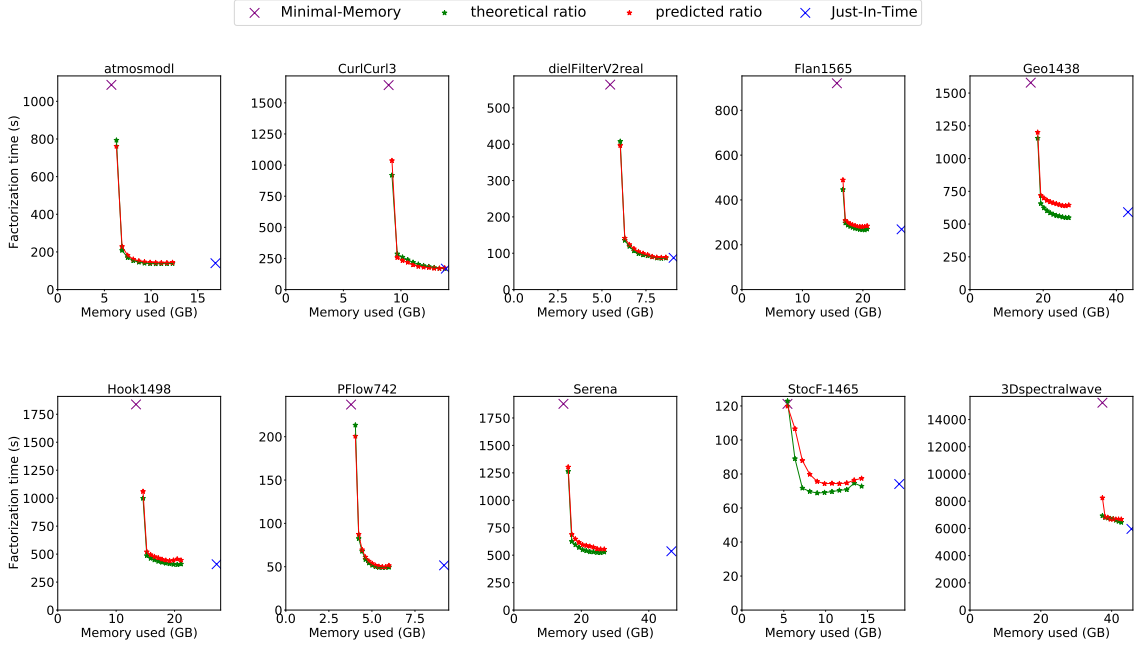
Figure 6: Memory/Performance trade-offs achievable with the proposed bi-objective strategy, compared to existing single objective strategies.
