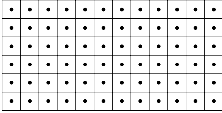
(a) The full space (in 2D) is separable with the given points.
