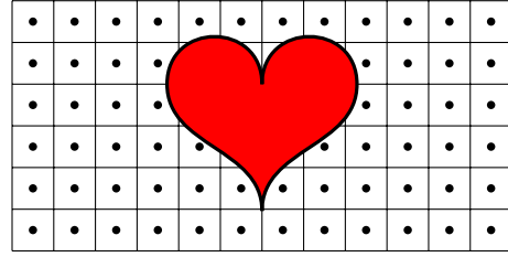
(b) The subset Y is heart-shaped. For ensuring its separability, we may provide points inside Y . But it is easier to only ensure weak separability by considering the same points as on the left, that may or may not belong to Y .
