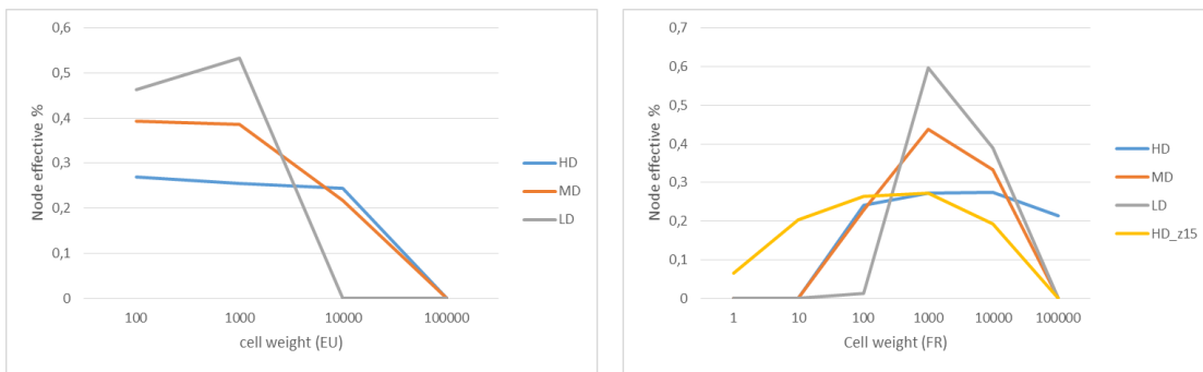
Figure 9. Node distribution by cell density in synthetic graphs (Left) Europe (Right) France. All curves used SFC zoom 12 except HD_z15 (Right) done with zoom 15.
