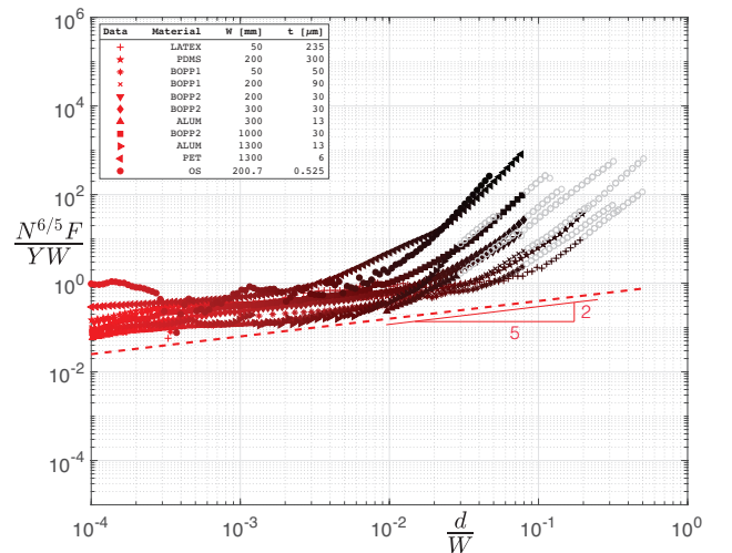
Fig. 4 Collapse of experimental data given in Fig. 2a (same color map) by using the dimensionless variables defined in Eq. (4). The red dashed line corresponds to Eq. (4) for c \approx 1 .
