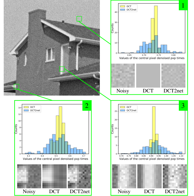
Fig. 7. For each noisy patch of size 13 \times 13 extracted from House image corrupted by AWGN with \sigma = 10 , its denoised version is displayed when processed by the original DCT and by the transform learned by DCT2net. The patches produced by DCT2net are very noisy compared to the original patches and patches denoised with DCT. Histograms show a comparison of the p^2 denoised values for the central pixel after transformation in each of the p^2 patches it belongs to ( p = 13 ). The variance of pixels intensities is higher with DCT2net.
