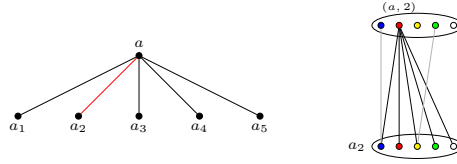
Figure 6.7: An example of graph G(5, m) with 5 colors. The conflict 5-graph of red edge aa_2 , when m = 5 , M_{aa_2} contains five black edges (a, 2)(a_2, i) for all i \in [5] ; and when m = 7 , then M_{aa_2} contains these black edges and two grey edges which are in the remaining edges of K_{aa_2}^5 .
