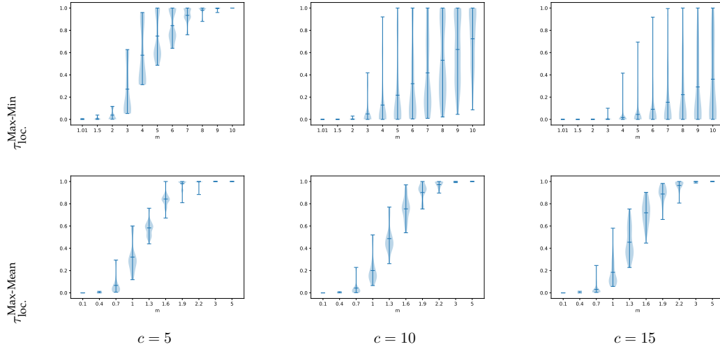
Figure 8.3: Violin plots for the fraction f_{c,m} of valid configurations in \prod_{p_i \in P} C[p_i] , for fixed values of the number of colors c and the multiplicative factors m in Equation 8.6. Each plot features three sub-plots corresponding to the number of colors c \in \{5, 10, 15\} ; each sub-plot features violins where each of which is corresponding to a multiplicative value in m_1 for \tau_{loc}^{Max-Min} , or m_2 for \tau_{loc}^{Max-Mean} . Each violin plot corresponds to R = 100 random instances. These experiments involve N' = 8 finite Voronoi regions.
