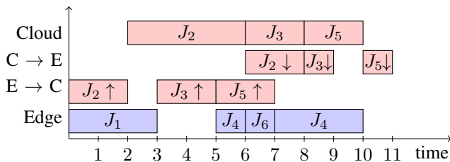
Fig. 1: Example of a valid schedule, with P^e = P^c = 1 .
