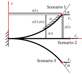
Fig. 8: The schematic beam deformation of Case 2
