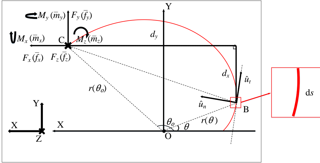
Figure 3: Loading conditions of an ICB for compliance analysis in X-Y plane
