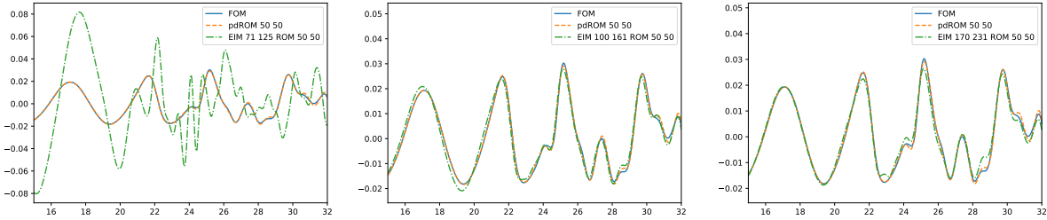
(d) EIM ROM simulation time-only reduction with N_{RB}^{\eta} = N_{RB}^q = 50 and tol_{EIM} = 10^{-4}, 3 \cdot 10^{-5}, 10^{-6} respectively from left to right
