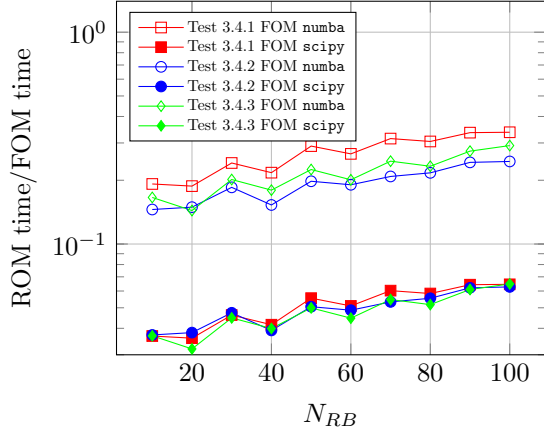
(a) Ratio between computational time of pdROM with respect to FOM computed either with Thomas solver in numba or with the sparse solver of scipy
