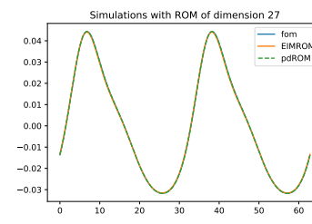
(l) ROM solutions time-parameter reduction with N_{RB} = 27 and N_{EIM} = 119 on parameter and \eta_0 outside the training set
