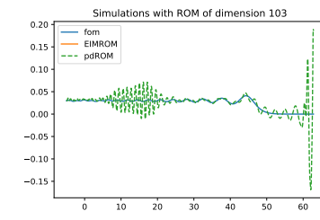
(l) ROM solutions time-parameter reduction with tol_{POD} = 0.0001 , N_{RB} = 103 on parameter and \eta_0 outside the training set
