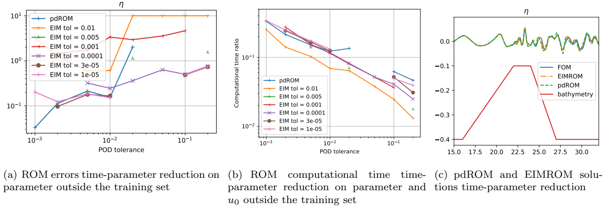
Figure 17: Monochromatic waves on a submerged bar. pdROM and EIM (time-parameter) reduction: simulation, errors and computational time, varying POD and EIM dimensions. Parameter outside the training domain.
