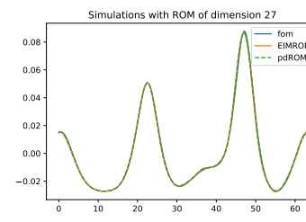
(k) ROM solutions time-parameter reduction with tol_{POD} = 0.3 , N_{RB} = 27 and tol_{EIM} = 0.0003 , N_{EIM} = 119 on parameter and \eta_0 in the training set
