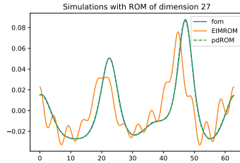
(h) ROM solutions time-parameter reduction with tol_{POD} = 0.3 , N_{RB} = 27 and tol_{EIM} = 0.03 , N_{EIM} = 72 on parameter and \eta_0 in the training set
