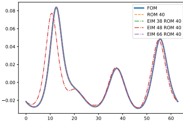
(j) ROM solutions time-only reduction
