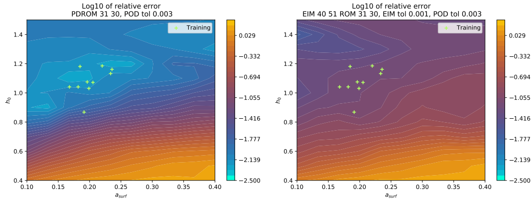
Figure 14: Solitary wave over a bar. Error plot varying the parameters a_0 and h_0 for pdROM N_{RB}^\eta = 31 and N_{RB}^q = 30 and EIMROM with N_{EIM}^\eta = 40 and N_{EIM}^q = 51
