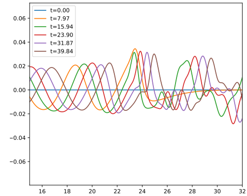
(d) Periodic waves over a submerged bar: \eta at different timesteps
