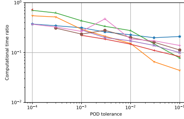
(e) ROM computational time time-parameter reduction on parameter and \eta_0 in the training set (legend above)
