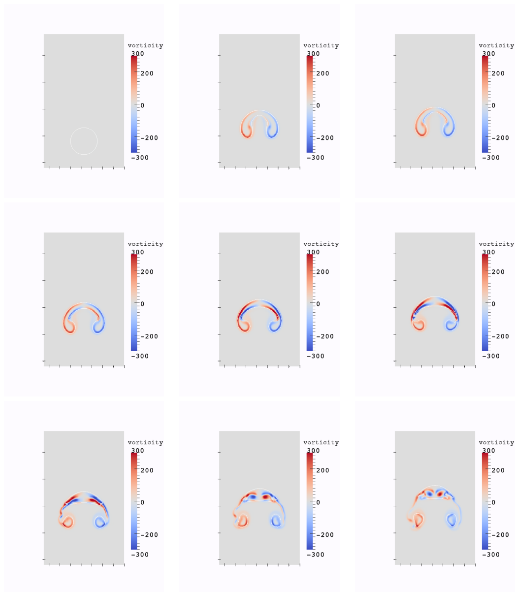
Figure 11. Evolution of the interface and vorticity values for the bubble test case from [36] at non-dimensional times t * \sqrt{-g/0.025} = 0., 2.8, 6, 4., 4.4, 4.8, 5.2, 5.6, 6. , resolution 120 \times 200 .
