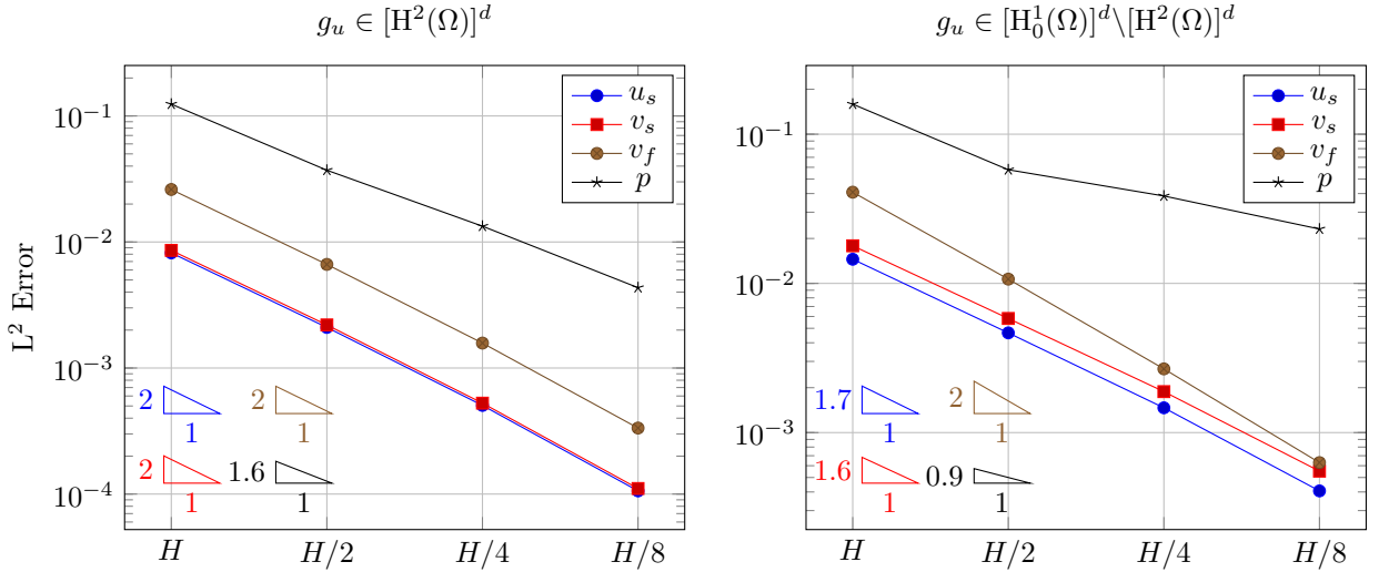
Figure 2: Approximation errors and computed convergence rates for the discretization of the incompressible ( \kappa = +\infty ) steady-state problem (76) with \mathbb{P}_1^b \times \mathbb{P}_1^b \times \mathbb{P}_1^b \times \mathbb{P}_1 elements.
