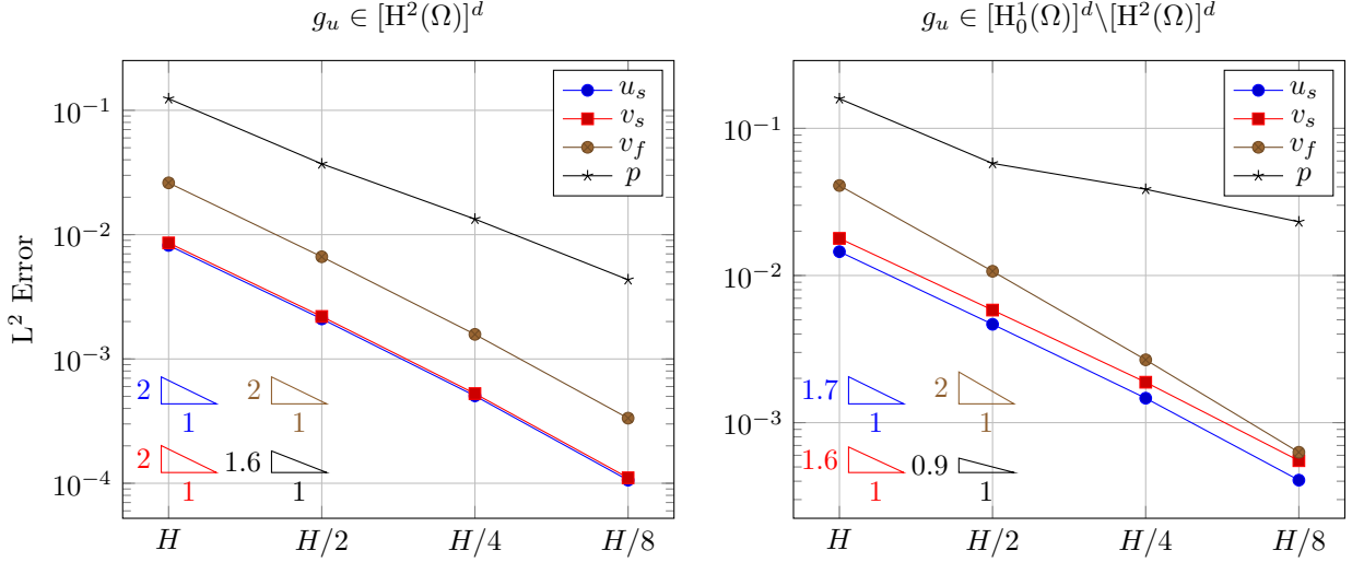
Figure 2: Approximation errors and computed convergence rates for the discretization of the incompressible ( \kappa = +\infty ) steady-state problem (95) with \mathbb{P}_1^b \times \mathbb{P}_1^b \times \mathbb{P}_1^b \times \mathbb{P}_1 elements.
