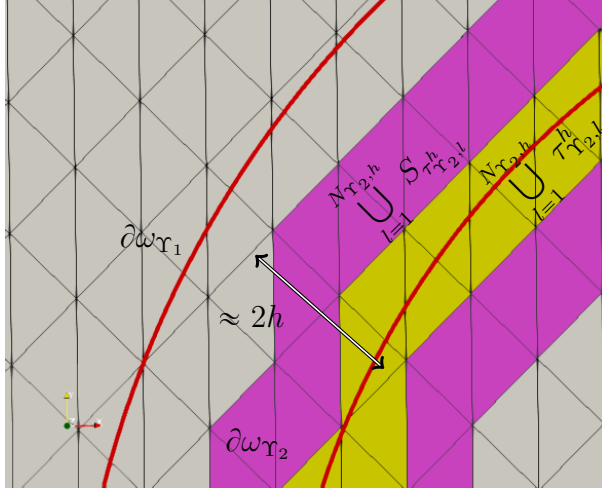
Figure 1: Geometric configuration of domain \omega_{T_2} and sets \left\{ \bigcup_{l=1}^{N_{T_2,h}} S_{\tau_{T_2,l}^h}, \bigcup_{l=1}^{N_{T_2,h}} \tau_{T_2,l}^h \right\} .
