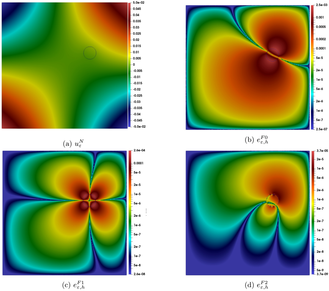
Figure 4: Contour plots of the solution u_\varepsilon and of the discrete model errors e_{\varepsilon,h}^{F0} , e_{\varepsilon,h}^{F1} and e_{\varepsilon,h}^{F2} on a log-scale axis for a circle of radius \varepsilon = 0.05 .
