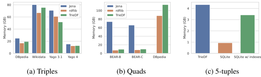
Fig. 3: Peek memory usage in gigabytes (GB)
