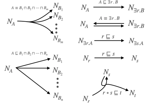
Figure 1: Illustration of hyper-edges.
