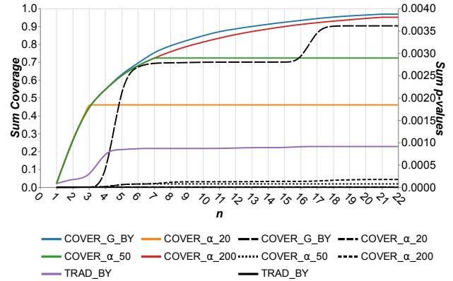
Figure 1: Coverage and p-values as a function of n
