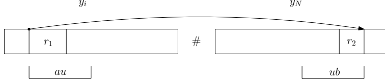
Figure 2: au starts where a word r_1 of R_{y_N}^\ell starts in y_i and ub ends where a word r_2 of R_{y_1\#\dots\#y_{N-1}}^\ell ends in y_N . Moreover, if |u| \geq \max\{|r_1|, |r_2|\} - 1 , then aub is a Case 2 MAW.
