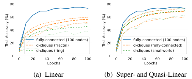
Figure 24. CIFAR10: D-Cliques convergence speed with 1000 nodes (10 nodes per clique, same number of updates per epoch as 100 nodes, i.e. batch-size 10x less per node) with different inter-clique topologies (variation of Figure 10 with 1 class/node instead of 2 shards/node).
