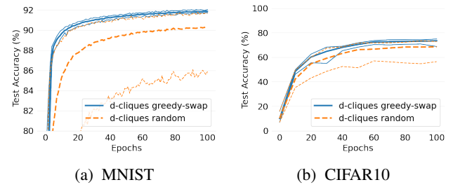
Figure 15. Convergence speed of D-Cliques constructed randomly vs Greedy Swap with 10 cliques of 10 heterogeneous nodes (100 nodes).
