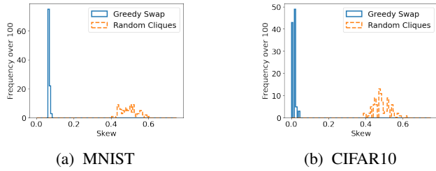
Figure 13. Final quality of cliques (skew) with a maximum size of 10 over 100 experiments in a network of 100 nodes.
