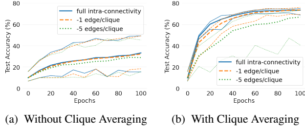
Figure 12. CIFAR10: Impact of intra-clique edge removal (with momentum) on D-Cliques (fully-connected) with 10 cliques of 10 heterogeneous nodes (100 nodes).
