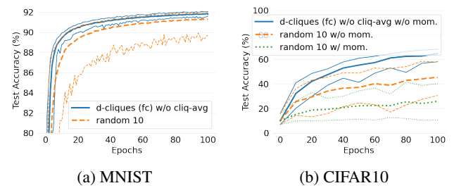
Figure 8. Comparison on 100 heterogeneous nodes between D-Cliques (fully-connected) with 10 cliques of size 10 and a random graph with 10 edges per node without Clique Averaging or momentum.
