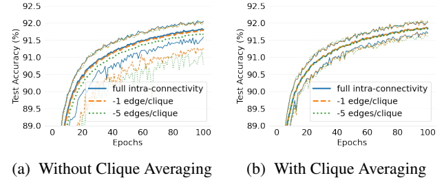
Figure 11. MNIST: Impact of intra-clique edge removal on D-Cliques (fully-connected) with 10 cliques of 10 heterogeneous nodes (100 nodes). Y axis starts at 89.
