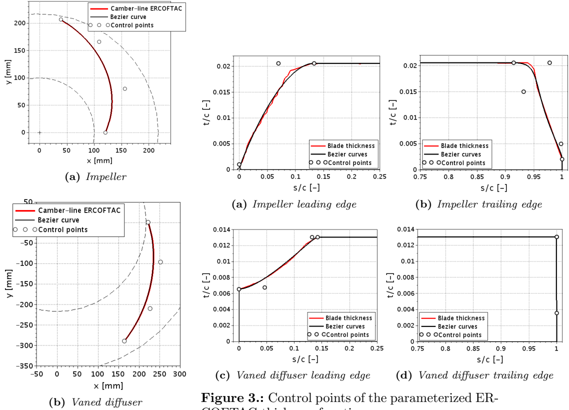
Figure 2.: Control points of the parameterized ERCOFTAC camber-lines
