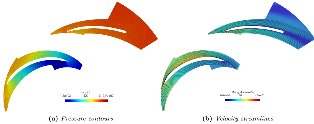
Figure 11.: Pressure and velocity fields of the SOGA optimized geometry
