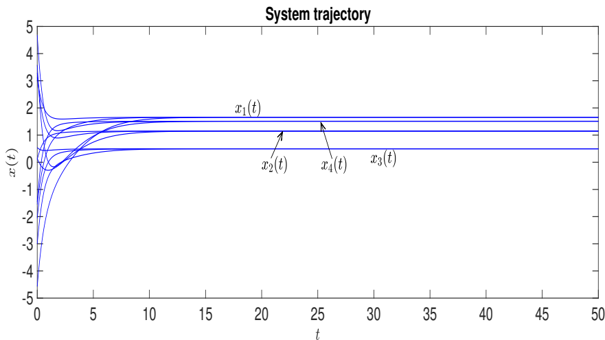
FIGURE 2 The state trajectories of (29) versus the time t
