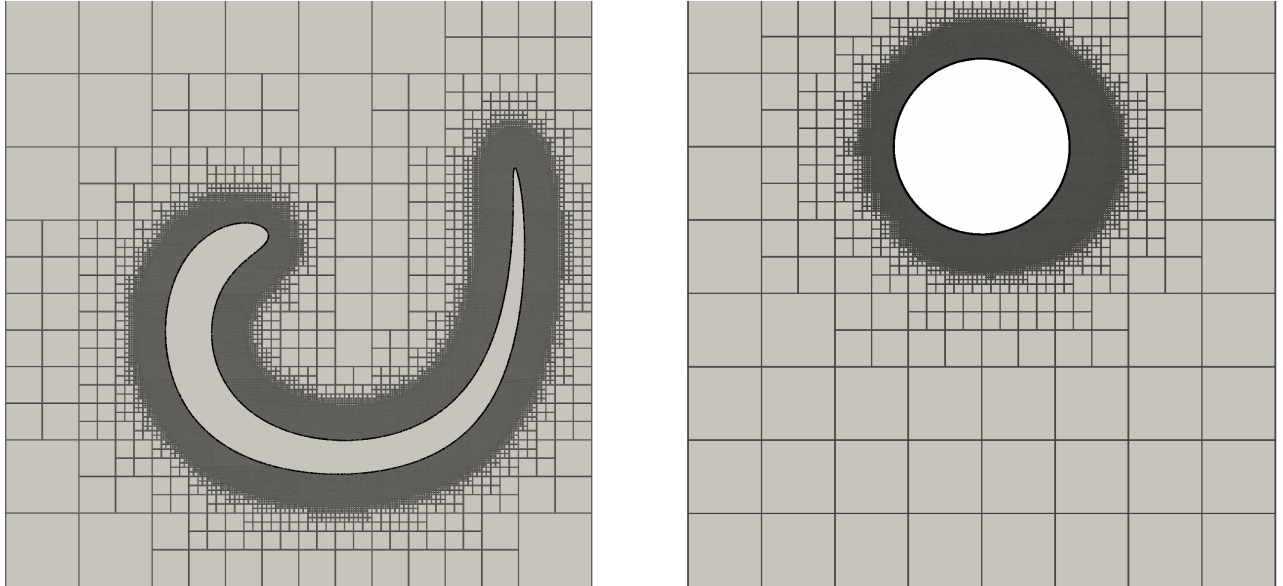
Figure 22: The serpentine: position of the interface at times t = T_{max}/2 (left) and t = T_{max} (right). The simulation was run on a dynamic quadtree mesh with L_{max} = 10 .
