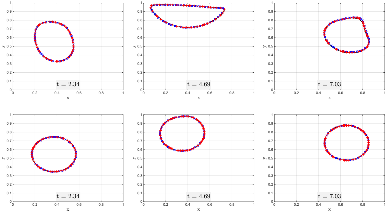
Figure 12: Deformation of soft (top range) and stiff (bottom range) solids immersed in a lid-driven cavity flow: interface location \Gamma_e for various time instants, comparison with the work of Zhao [57] (black line). The blue-plus and red-cross markers refer to the results obtained on uniform L_9 and L_{10} grids respectively.
