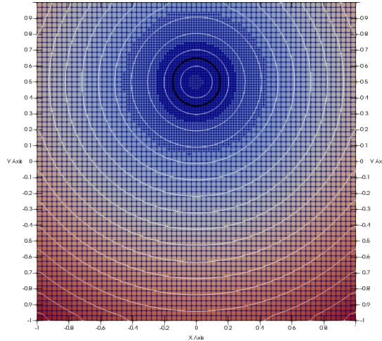
Figure 21: Advection of a circle: contours of the level-set function (the interface is drawn in black) and the quadtree mesh L_6 - L_8 at time t = T_{max} .
