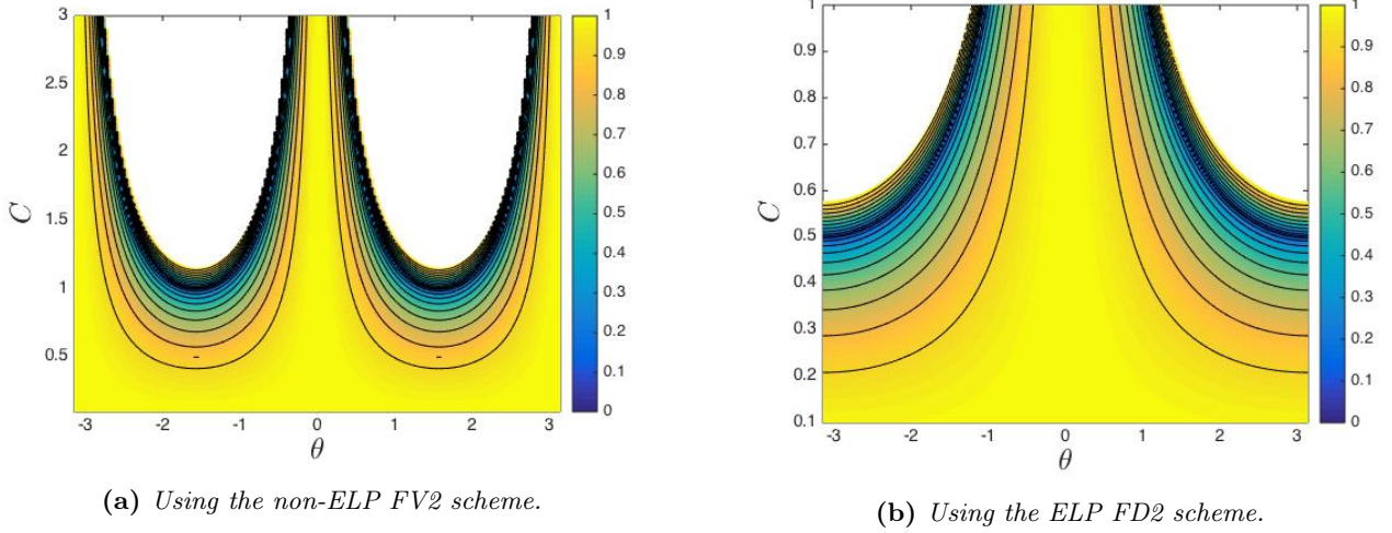
Figure 9: Asymptotic analysis of the model (38): amplification factors as a function of the frequency of a Fourier mode \theta and the CFL number C = a\Delta t/\Delta x obtained using ELP and non-ELP discretizations of the advective term A(Y) . Inside the white regions, the amplification factor is greater than 1.
