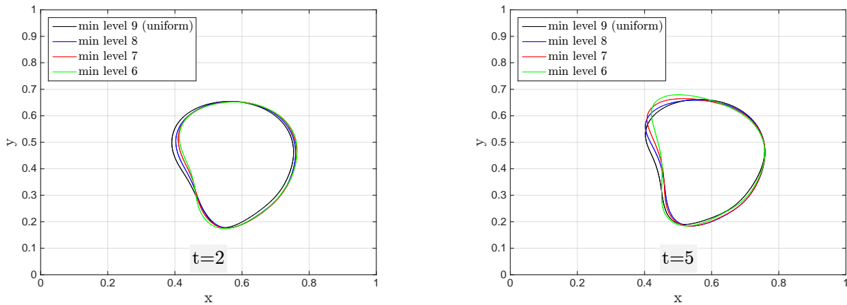
Figure 16: Solid deformation due to an immersed actuator: position of the interface \Gamma_e(t) at time t = 2 (left) and t = 5 (right). The comparison is performed between the L_9 uniform grid and dynamic AMR grids for a same maximum level of refinement L_{max} .
