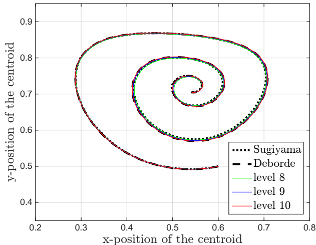
Figure 13: Deformable soft solid ( G = 0.1Pa ) in a lid-driven cavity flow: approximated centroid position over time until t = 20s . The simulations are run on L_8 to L_{10} uniform grids. The centroid position is computed following Eq. 58.
