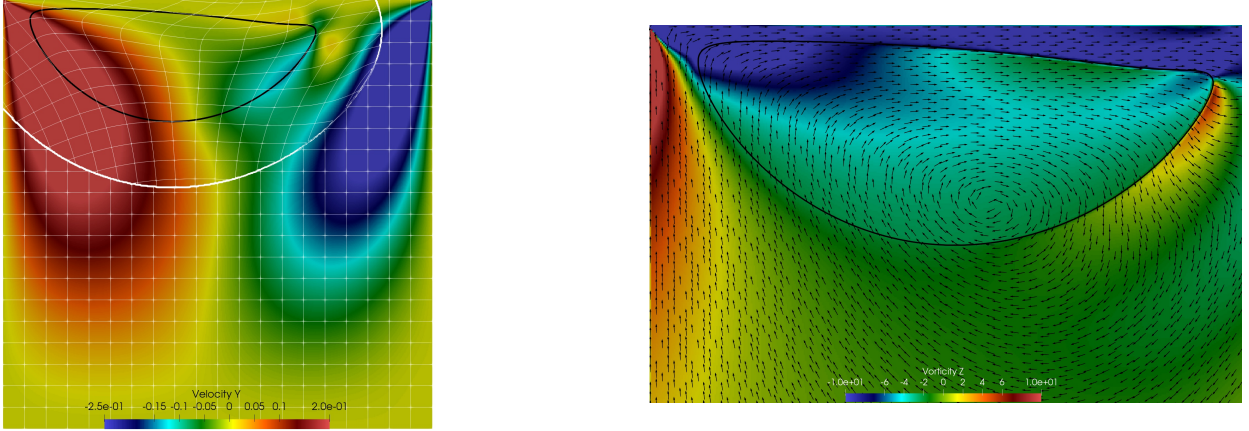
Figure 11: Deformable soft solid ( G = 0.1\text{Pa} ) in a lid-driven cavity flow: snapshots at time t = 4.69\text{s} . Left: y -component of the velocity; right: z -component of the vorticity with velocity field. The black and white lines represent the interface \Gamma_e and the contours of the backward characteristics \mathbf{Y} respectively. The discontinuity of the characteristics is due to the extrapolation process which is only performed up to a certain distance from the interface.
