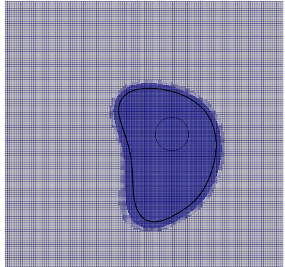
(b) dynamic AMR L_7 - L_9 grid
