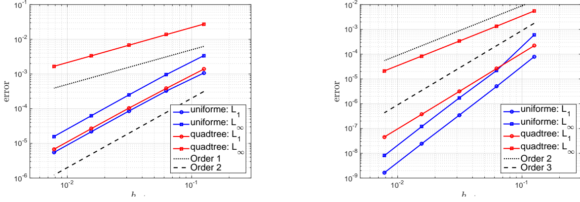
(a) With a linear interpolation of the fluxes + a mid-point quadrature rule.
