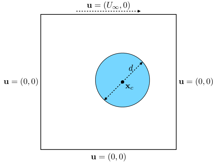
Figure 10: Deformable solid in a lid-driven cavity flow: fluid-structure set-up.
