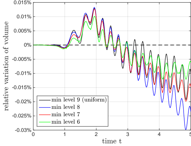
Figure 17: Solid deformation due to an immersed actuator: estimation of the relative mass-conservation error over time. The comparison is performed between the L_9 uniform grid and dynamic AMR grids for a same maximum level of refinement L_{max} .
