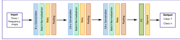
Figure 3: Representation of the neural network architecture (2DTF-VGG).
