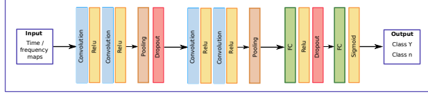
Figure 2: Representation of the neural network architecture (2DTF-CNN).
