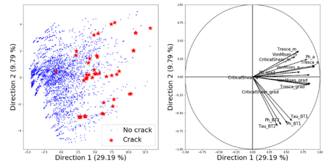
Figure 4: First and second principal components and correlation circle
