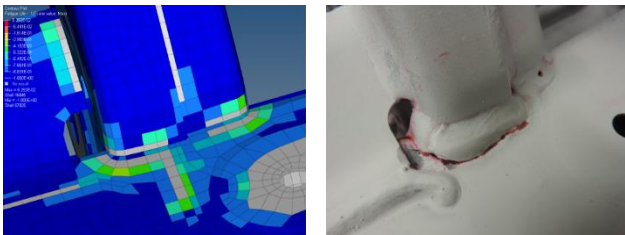
Figure 1: Crack initiation on a welded joint (right) and corresponding zone on the numerical model (left)
