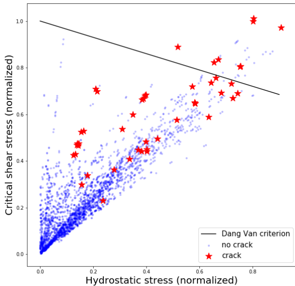
Figure 3: ph - \tau Dang Van diagram: from the bench tests, we observe cracks (represented as red stars) on areas predicted to be safe by the Dang Van criterion.
