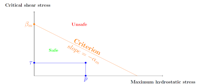
Figure 2: Dang Van criterion. A zone is safe (resp. unsafe) if (ph, \tau) below (resp. above) the straight line.
