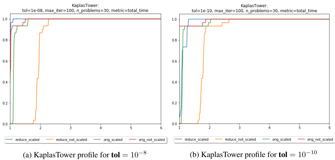
Figure 4.10: KaplasTower problem (no sliding).
