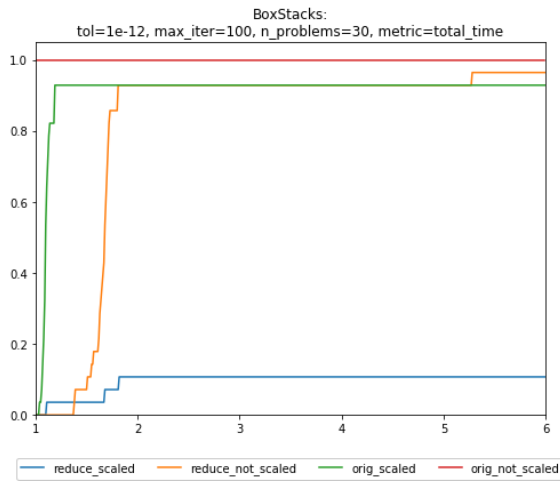
Figure 4.9: (c) BoxStacks profile for \text{tol} = 10^{-12}
