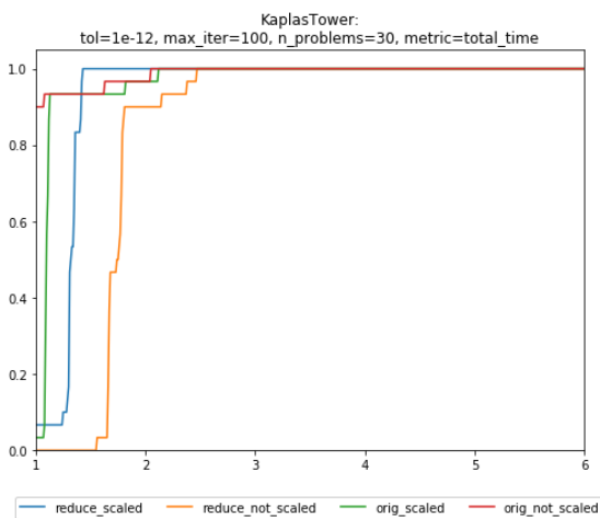
Figure 4.12: (c) KaplasTower profile for \text{tol} = 10^{-12}
