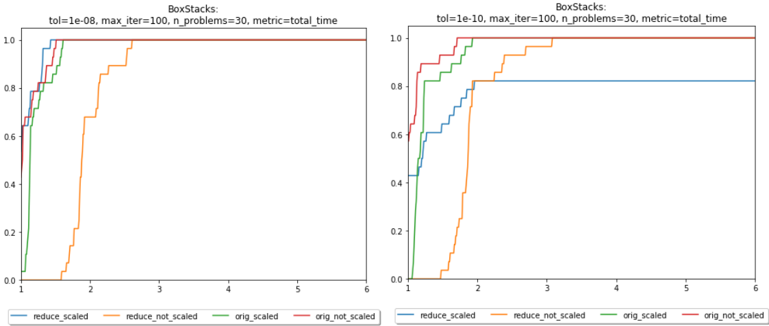
(a) BoxStacks profile for \text{tol} = 10^{-8}
