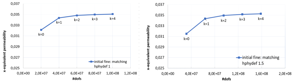
Figure 7: x -equivalent permeability versus #dofs. Left: L150; right: L200.
