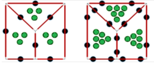
Figure 5: Discrete unknowns in three mesh cells. Here, the order of the cell polynomials is l = k + 1 , and k is the order of the face polynomials. (left) k = 0 and (right) k = 1 where black dots are the face unknowns and green dots are the cell unknowns.
