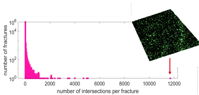
Figure 2: L200: histogram of the number of intersections per fracture.
