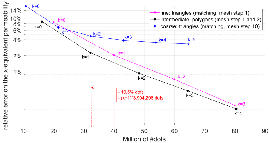
Figure 14: L150: relative error on the x -equivalent permeability versus the number of dofs. Example of gain obtained with a polygonal discretization.
