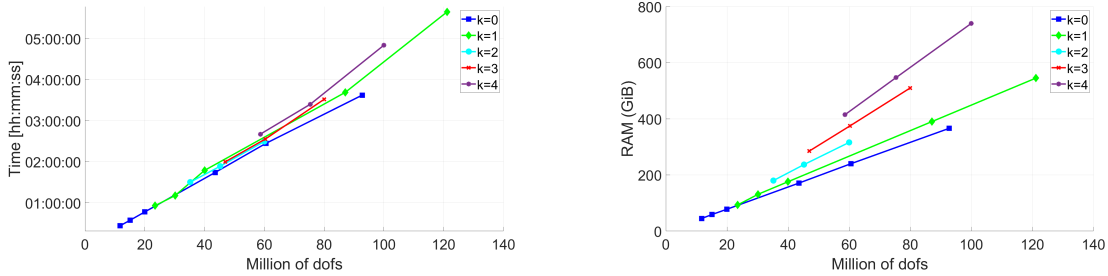
Figure 10: L150: computational time (left) and RAM requirements (right) versus the number of dofs.
