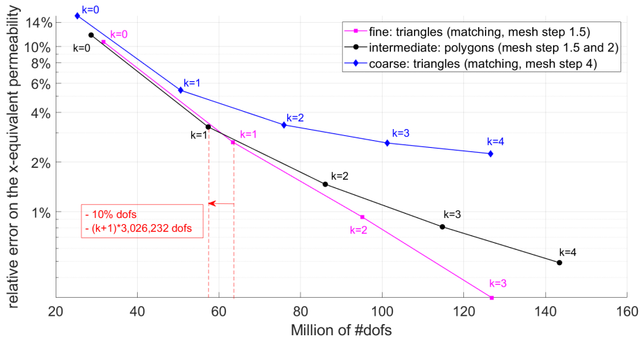
Figure 15: L200: relative error on the x -equivalent permeability versus the number of dofs. Example of gain obtained with a polygonal discretization.
