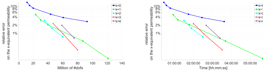
Figure 8: L150: relative error on the x -equivalent permeability versus the number of dofs (left) and versus computational time (hh:mm:ss, right).
