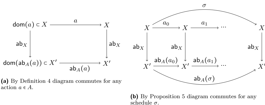
■ Figure 1 ( ab_X, ab_A ) forms an abstraction between the POTS (X, \subseteq, A) and (X', \subseteq, A') .
