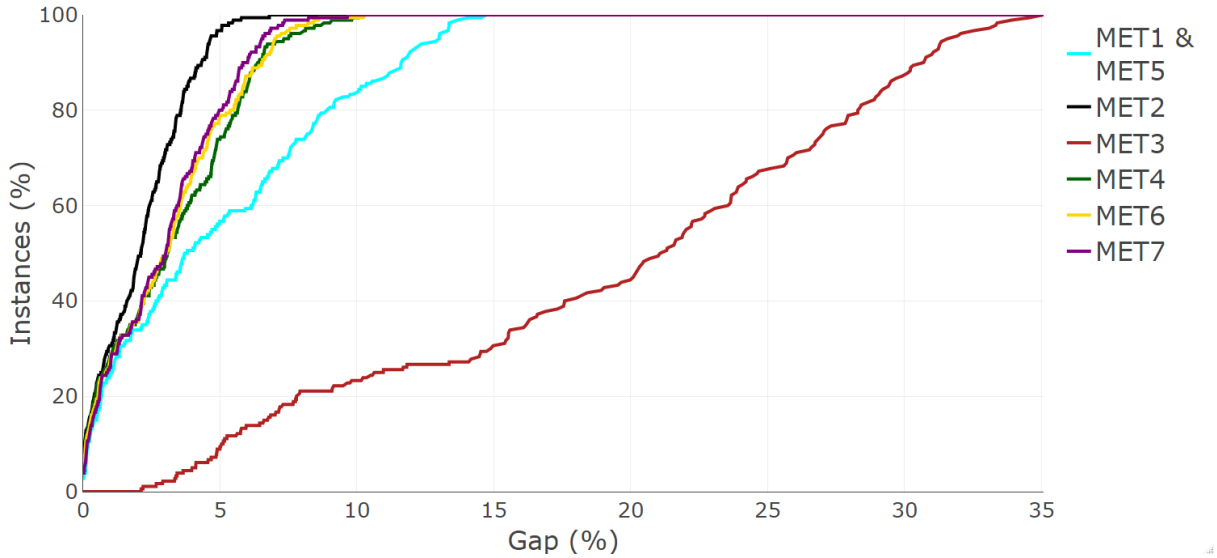
Figure 2: In the y -axis, the percentage of instances with an integrality gap less than or equal to that of the x -value is represented for MET1-MET7
