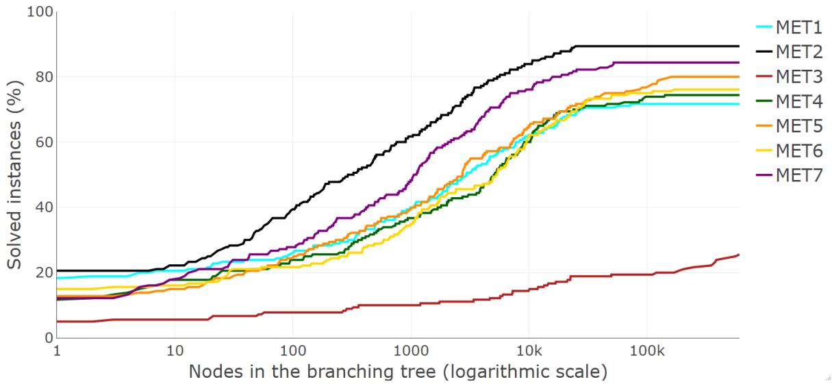
Figure 3: In the y -axis, the percentage of instances solved exploring an amount of nodes in the branching tree less than or equal to that of the x -value is represented for MET1-MET7
