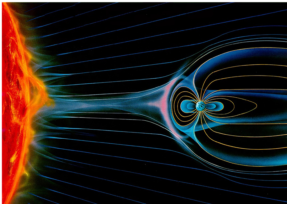
Fig. 1. Radiation effects from the Sun-Earth relationship [19].
