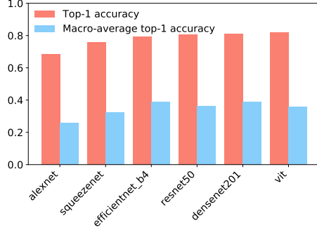
Figure 5: PI@ntNet-300K test top-1 accuracy and macro-average top-1 accuracy for several neural networks.
