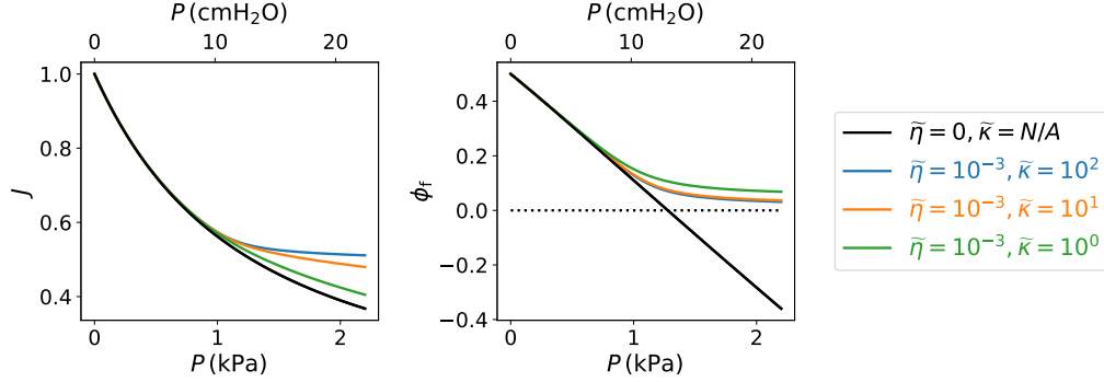
(a) Influence of the solid bulk modulus \tilde{\kappa} when using the pore energy \widetilde{W}_{\text{por}} . As long as the porosity is away from zero, the solid bulk modulus has little impact, since the volume decrease is mainly due to air ejection and less to solid compression. Then, when the porosity comes close to zero, the solid starts to be compressed according to the solid bulk modulus.
