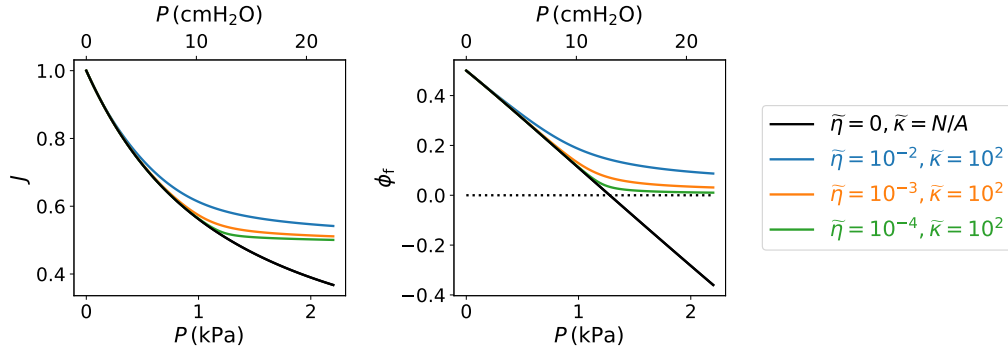
(b) Influence of \tilde{\eta} when using \widetilde{W}_{\text{por}} . When \tilde{\eta} decreases, the change of behavior when the porosity comes close to zero becomes sharper.
