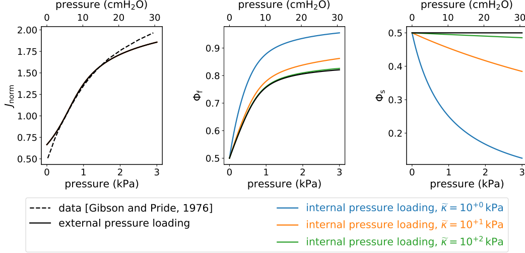
Figure 2: Mechanical response of the mixture resulting from our choice of \widetilde{W}_{\text{skel}} in Eq. (27) & \widetilde{W}_{\text{bulk}} in Eq. (29) for various values of bulk modulus \tilde{\kappa} (while other parameters are fixed at \Phi_{f0} = 0.5 , \tilde{\alpha} = 0.16 kPa, \tilde{\beta}_1 = 0.2 kPa, \tilde{\beta}_2 = 0.4 kPa & \delta = 0.5 ) and applied pressure – positive when internal or negative when external, here considered in absolute value in the plots. The solid black curve corresponds to an external negative pressure loading ( i.e. , by imposing \underline{\Sigma} > 0 and p_f = 0 , in which case the response only depends on \widetilde{W}_{\text{skel}} , not \widetilde{W}_{\text{bulk}} , hence not on \tilde{\kappa} ), while the colored curves correspond to a positive internal pressure loading ( i.e. , by imposing p_f > 0 and \underline{\Sigma} = 0 , in which case the response depends on \tilde{\kappa} , so various values are considered). All curves are obtained by imposing a level of pressure and solving the nonlinear behavior law at one single material point – i.e. , a Rivlin cube – through a Newton-Raphson procedure, in order to compute the associated mixture deformation & volumes fractions changes. (Left) Volumetric response of a mixture to a pressure loading, compared to experimental data [Gibson and Pride, 1976]. J_{\text{norm}} is the mixture volume change J normalized by its value at 0.5 kPa (which roughly corresponds to the end-exhalation state in the lung model), leading to J_{\text{norm}} = J/J_{0.5} = 1 for an applied pressure of 0.5 kPa. The colored curves are superimposed with the black curve because the mixture volume deformation is identical for internal vs. external applied pressure. (Center & Right) Evolution of the volume fraction of fluid ( i.e. , the porosity) and solid with the pressure loading. When the mixture is subjected to internal pressure, the solid phase is compressed according to its bulk modulus; the lower the bulk modulus, the more compressible the solid, the higher the volume fraction of fluid and the lower the volume fraction of solid. For the value of the bulk modulus used in the rest of the paper ( \tilde{\kappa} = 10^2 kPa) the change in solid volume is very limited.
