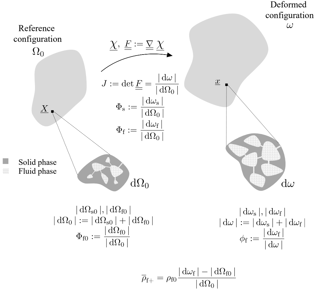
Figure 1: Schematic of the reference and deformed configurations with associated local quantities, volumes and porosity. \mathrm{d}\Omega_0 , \mathrm{d}\omega , \mathrm{d}\Omega_{f0} , \mathrm{d}\omega_f , \mathrm{d}\Omega_{s0} , \mathrm{d}\omega_s are the infinitesimal volumes of the mixture, the fluid and solid phases, in the reference and deformed configurations, respectively. \Phi_{f0} and \phi_f are the porosities in the reference and deformed configurations, respectively. \bar{\rho}_{f+} is the added fluid mass density defined in the reference configuration. J , \Phi_s , \Phi_f are the local volume ratios.
