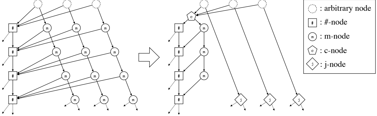
Figure 3: An example of contracting a part of the decision DAG. Before contracting, there are three parallel m -paths each of length 2^2 = 4 . We contract each m -path to a j -node corresponding to the case in which four consecutive non-sensitive patterns are merged. Also, we create an m -path of length 3 preceded by a c -node corresponding to the case in which at least one gadget is inserted.
