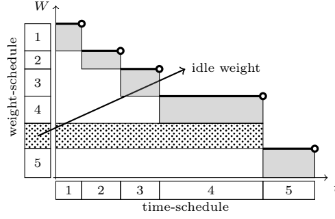
Fig. 1. 2D-Gantt chart. The x-axis shows a time-schedule, while the y-axis corresponds to W(t) = \sum_{C_j > t} w_j plus the idle weight in the corresponding weight-schedule [17].
