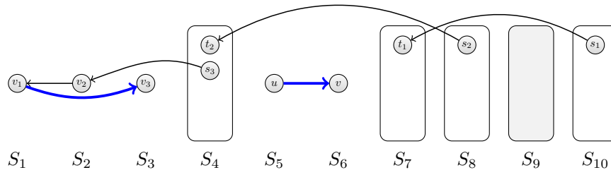
Figure 6: A nice decomposition of a strong semicomplete digraph with four backwards arcs (in thin black). The arc uv is regular-compulsory. The arc v_1v_3 is left-compulsory.
