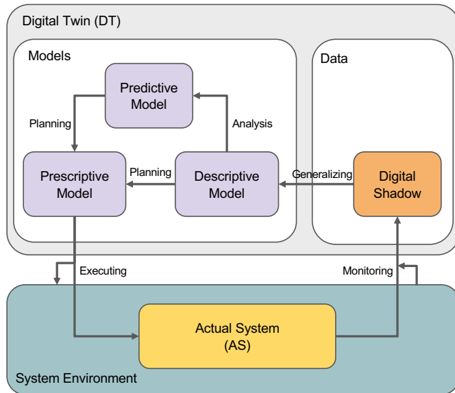
Fig. 1: Conceptual framework for DTs based on MODA [3]
