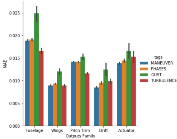
Fig. A.1: Prevision IO: Performance by family of outputs and flight sequence classes.
