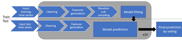
Fig. A.2: Amiral Technologies: System overview.
