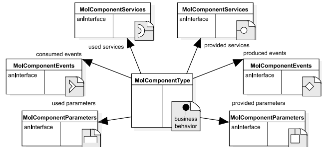
Fig. 5 Component contract implementation in Molecule.
