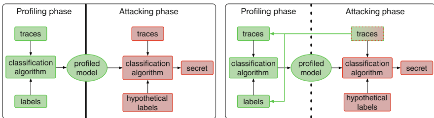
Fig. 8.2 Profiling side-channel scenario: supervised (left), semi-supervised (right)
