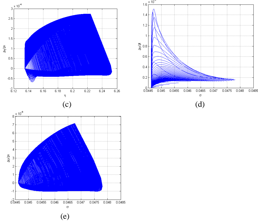
Fig. 1. The density temporal evolution and phase plane diagrams with initial homogeneous traffic of amplitude \rho_0 = 0.037 \text{ veh/m} (a) the temporal evolution of vehicle density; (b) the phase plane diagram of (\eta, \frac{\partial \eta}{\partial t}) ; (c) the phase plane diagram of (\eta, \frac{\partial \eta}{\partial x}) ; (d) the phase plane diagram of (\sigma, \frac{\partial \sigma}{\partial t}) ; (e) the phase plane diagram of (\sigma, \frac{\partial \sigma}{\partial x})
