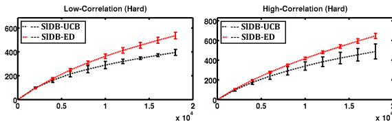
Figure 3: Regret ( R_t ) vs time ( t ) over availability sequences S_T
