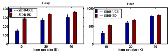
Figure 4: Final regret ( R_T ) at T = 10^4 with varying sizes ( K )
