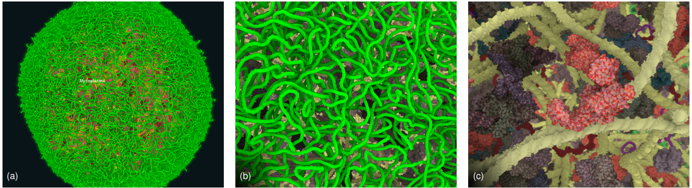
Fig. 9. The Mycoplasma model contains many more fiber instances (a). Throughout the virtual tour we visit both the strands visible from the outside view (e.g., peptides shown in (b)) as well as the insides of the bacterium pictured in (c).
