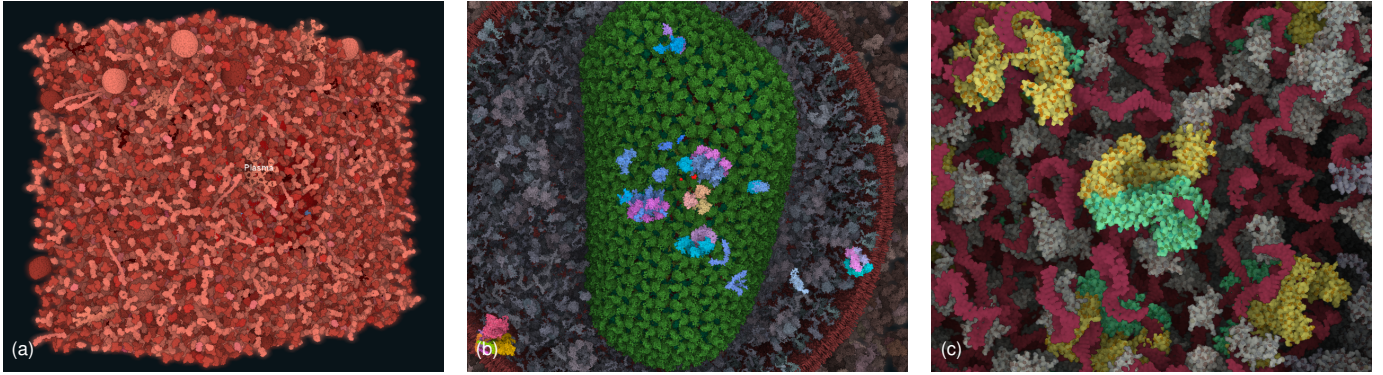
Fig. 1. In the tour of the HIV in blood plasma model (a) we, for example, visit the capsid (b) which contains the genetic information of the virus. Besides the RNA, the capsid contains several important proteins, such as Reverse Transcriptase (c).
